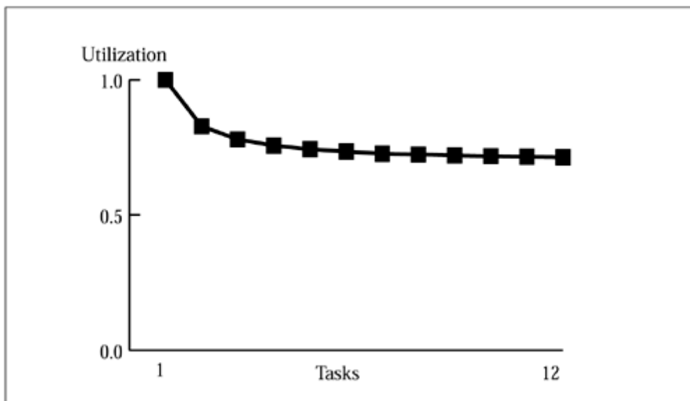
Figure 7-1. RMA efficiency
