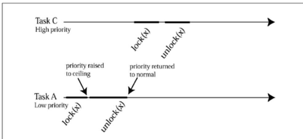
Figure 5-5. Priority ceiling emulation
